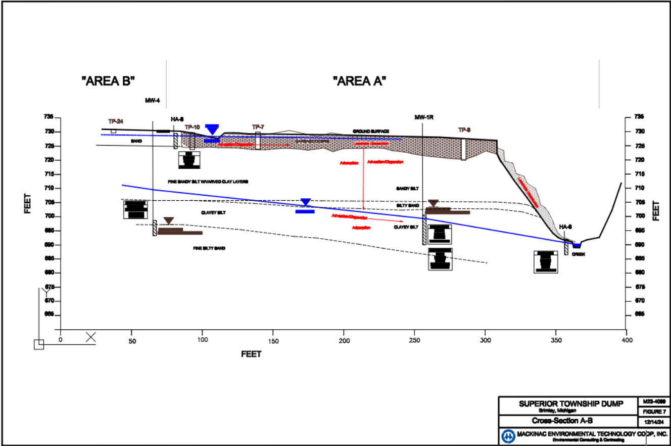
Figure 7 - Cross-Section A-B
